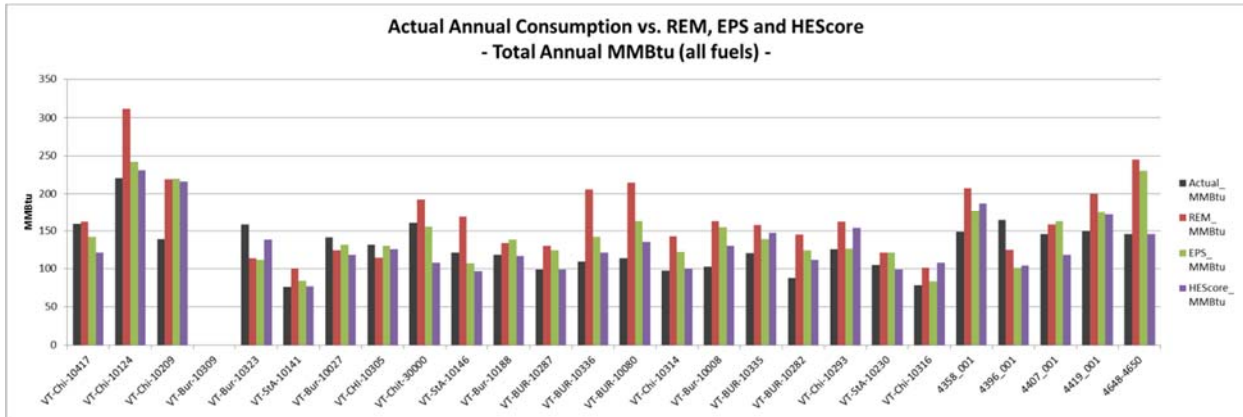
Figure 11. Quantitative Analysis of 26 Vermont Homes – Actual vs. Modeled Consumption (MMBtu Total of All Fuels)
